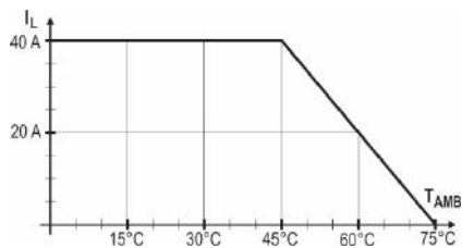
Figura 3 – SSR4840 + dissipador ND40-100 mm
