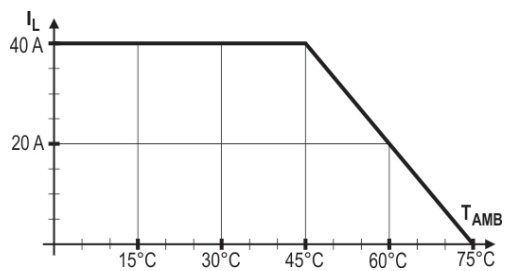
Fig. 5 – SSR4840 + dissipador ND40-100 mm
